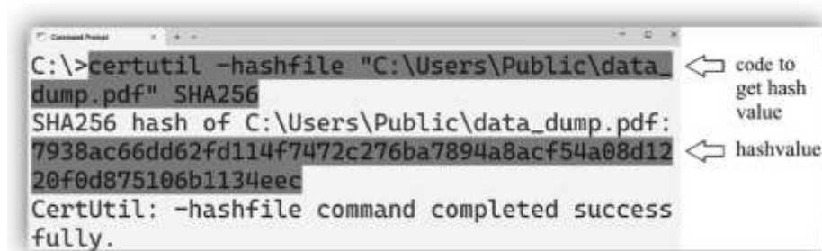
Fig. An illustration for generation of a SHA256 hash value of a (.pdf) file using command prompt.
