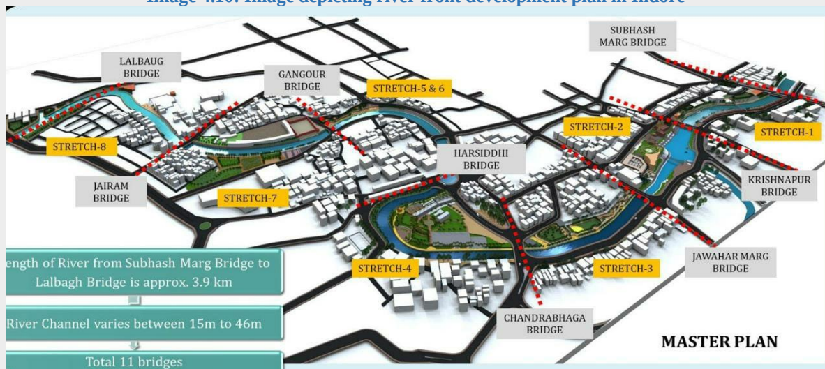
Image 4.10: Image depicting river front development plan in Indore
