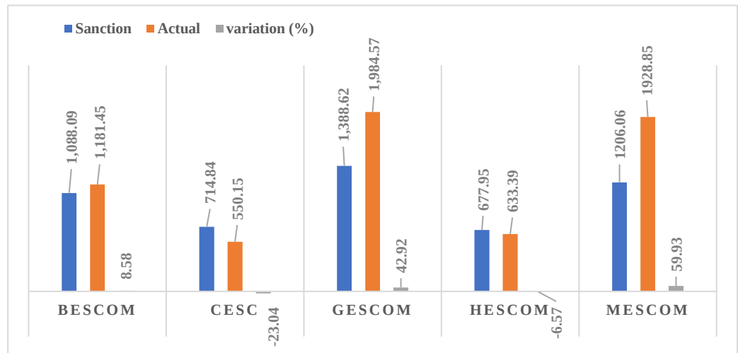
Chart No. 2.1 (b): Percentage of actual quantities executed (LT lines – CKMs) over sanction under DDUGJY
